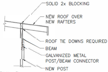
⊕ DETAIL D NTS
