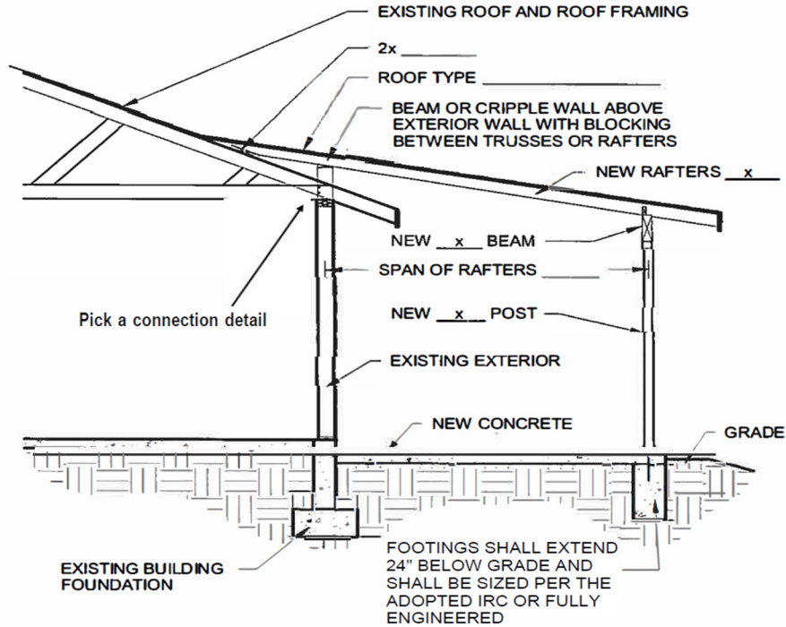
① SECTION THRU BUILDING 1/4" = 1'-0"
